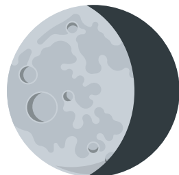
Waning Gibbous
