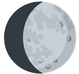
Waxing Gibbous
