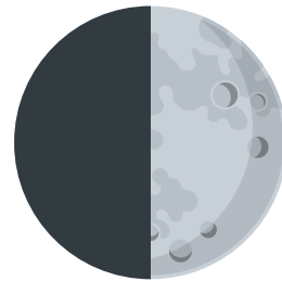
Waxing Quarter
