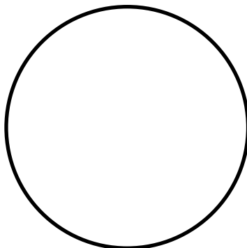
Last Quarter
