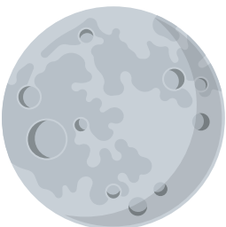
Full
