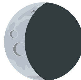
Waning Crescent
