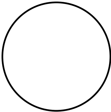
New moon
