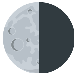
Waning Quarter
