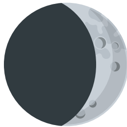
Waxing Crescent
