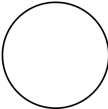
Full Moon
