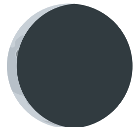
Old
