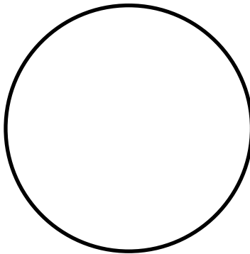
Waxing Crescent
